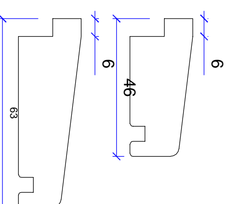
FRAME EXTENSION CILLS
