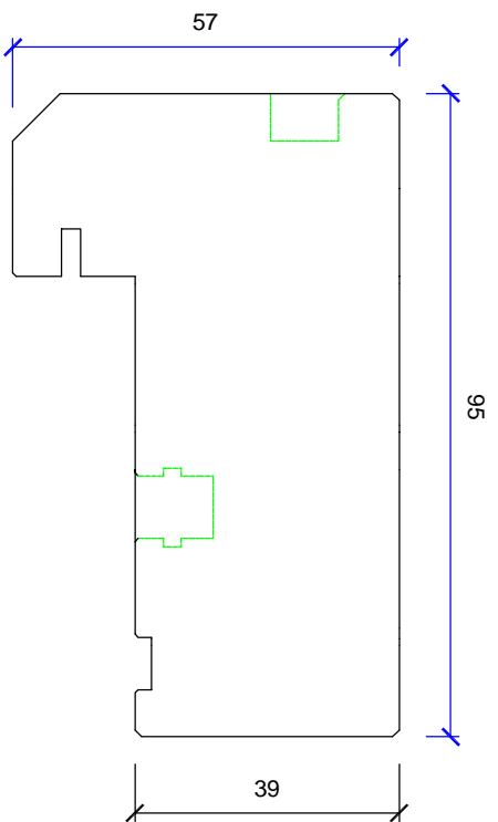
FRAME HEAD
