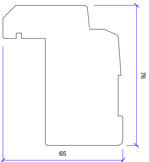
SASH STILE
