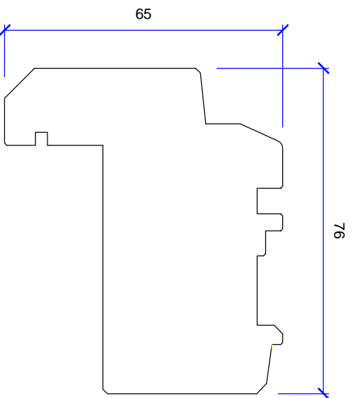
SASH TOPRAIL
